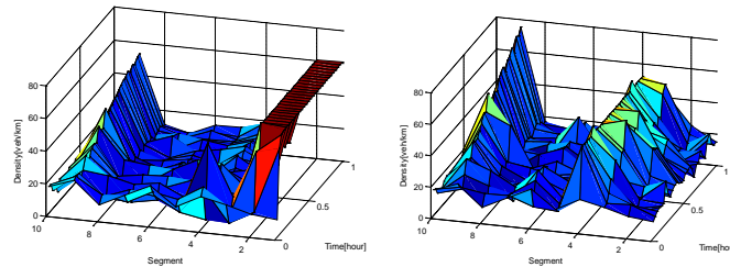
Figure 6.8 Density History of Scenario 1 for 4500 veh/h Demand at Origin. Left: Speed limit signs are controlled by the rounded optimal solution. Right: Uncontrolled case with desired speed of 120km/h for each segment.
