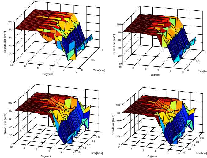
Figure 6.7 Histories of Controlled Speed Limit. Upper Left: 4500 veh/h Demand at Origin. Upper Right: 5000 veh/h Demand at Origin. Lower Left: 5500 veh/h Demand at Origin. Lower Right: 6000 veh/h Demand at Origin.
